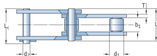
with small rollers
