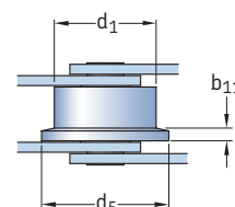
with F flanged rollers
